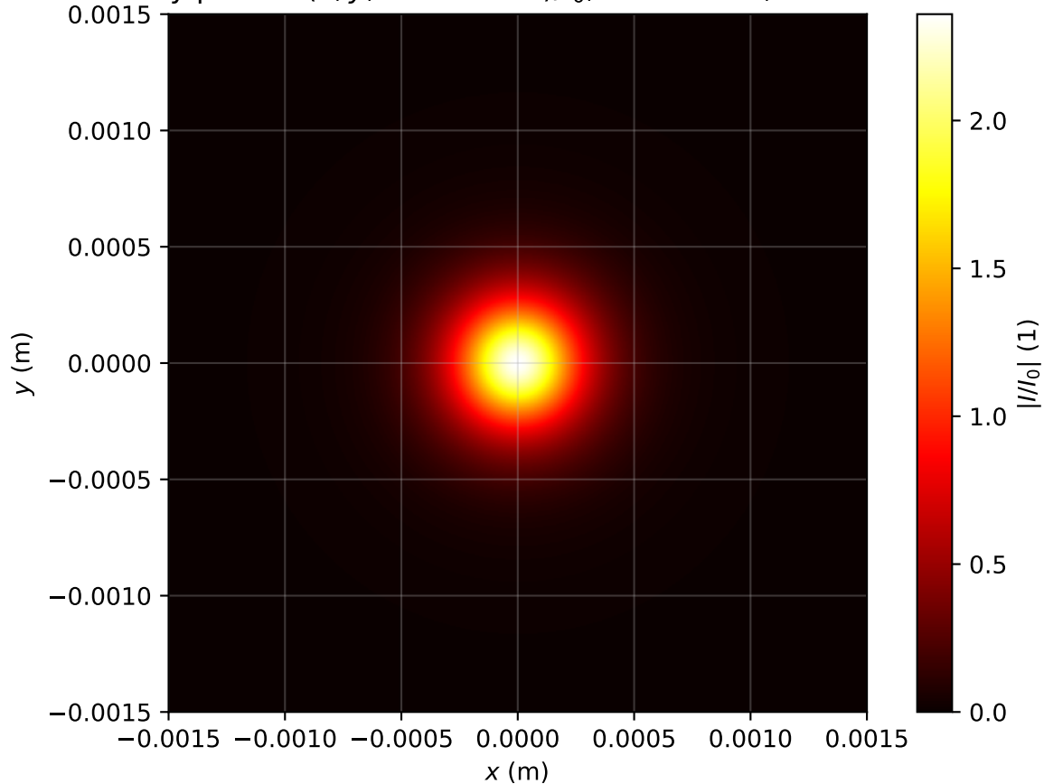
Intensity profile I(x, y, z = 2.468m)/I_0 , Pin=1.0Pcr, artificial time
